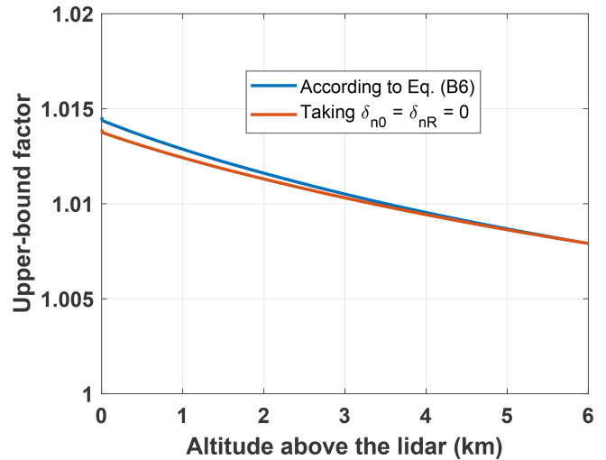
Figure B1. Upper-bound factor of the overlap function obtained with the wavelength combination 532–607 nm for the measurement of 1 December 2021, assuming a 50 sr aerosol lidar ratio, a 0.05 aerosol optical depth and a 1.3 maximum Ångström exponent.
