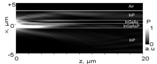
Figure 1: 2D-BPM modeling of light propagation issued from a lensed fiber in a waveguide HPT with a quaternary subcollector.
