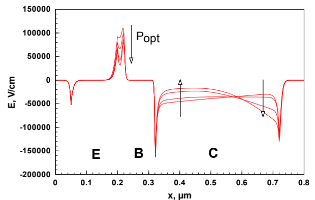
Figure 2: modeled electrical field in a HPT for various incident optical powers (0, 1, 5 and 10 mW). V_{ce}=1.5 V, I_b=10 \mu A, \lambda=1.55 \mu m.
