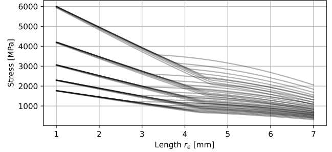
Fig. 12 Set of curves presenting the maximum stress \sigma_{max} as a function of r_e , plotted for \tau_{out}^{max} = 600 N.mm, R_a = 10 mm, and all pairs ( R ; r_s ) such that R \in \{1.5, 2, 2.5, 3, 3.5, 4, 4.5, 5.0\} mm and r_s \in \{0.4, 0.45, 0.5, 0.55, 0.6\} mm
