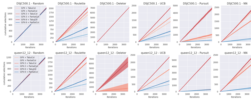
Fig. 2. Average cumulative selections, along with error bars, for each pair of operators based on different criteria on the DSJC500.1 and queen12_12 instances.
