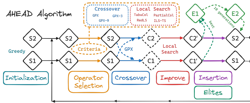
Fig. 1. General architecture of the Adaptive HEAD (AHEAD) framework.
