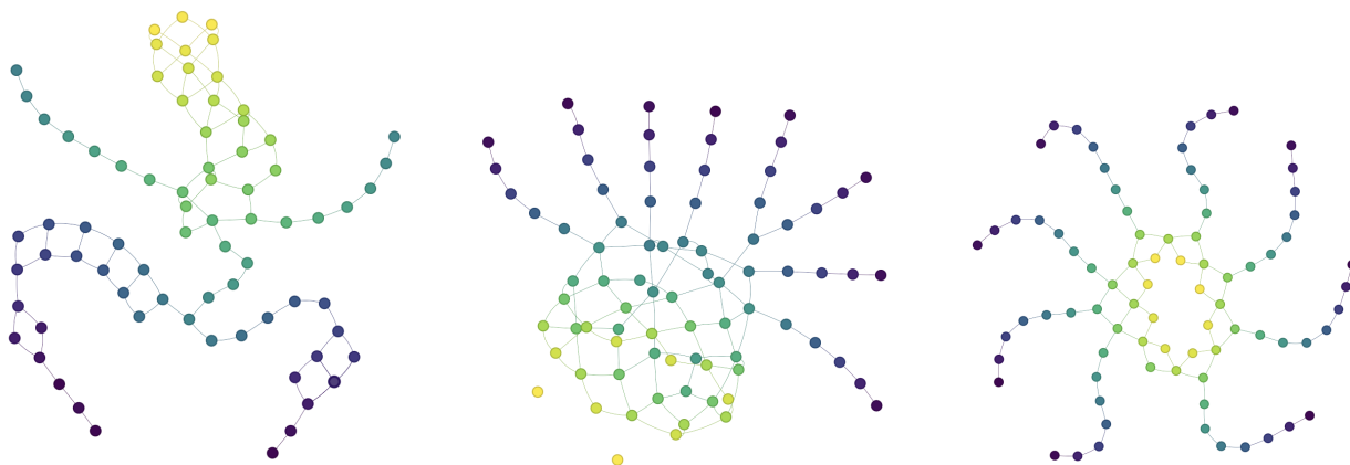
Figure 4: Regular Mapper graphs computed with the optimized filter function, corresponding, from left to right, to: the human, the octopus and the table. Vertices are colored using the mean value of the filter function in the corresponding clusters.
