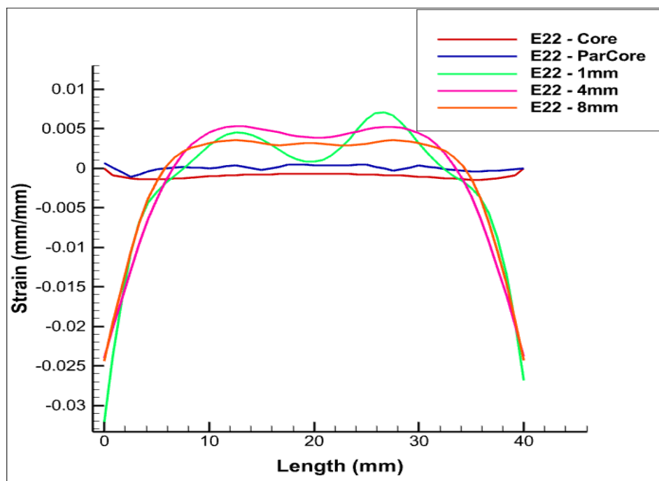
Figure 7. E_{yy} Eyy for various positionings of FOS in the case of the pure bending test case, along y axis.
