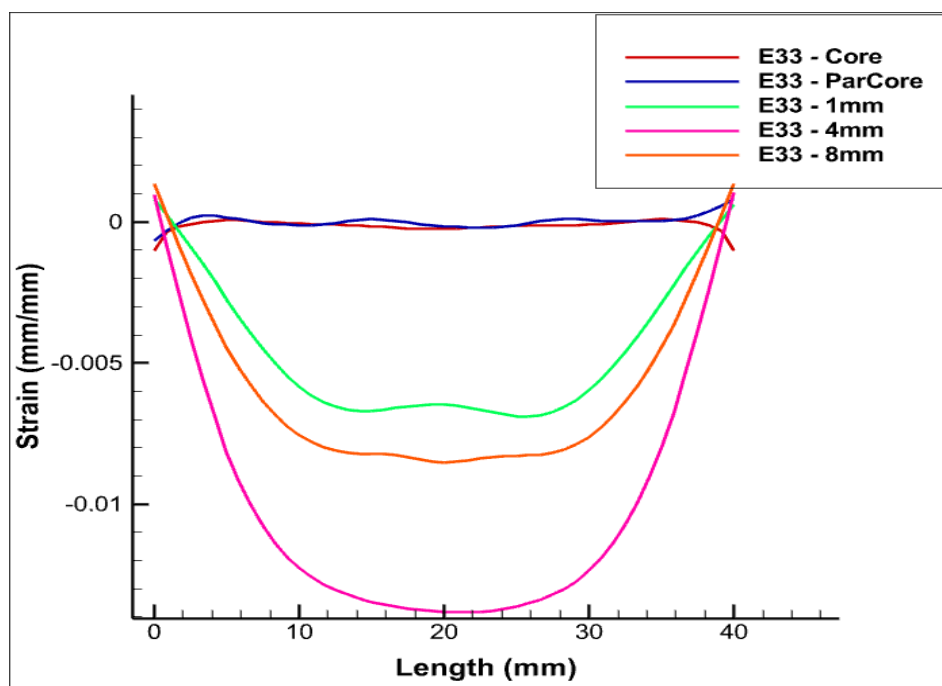
Figure 8. E_{zz} Ezz for various positionings of FOS in the case of Pure Bending Test Case, along z axis.
