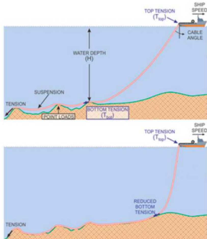
Figure 1. An example of the steep and sloppy topography at the bottom sea [25].
