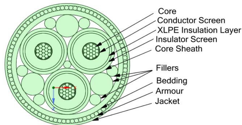
Figure 2. Cross-section of the cable [1].
