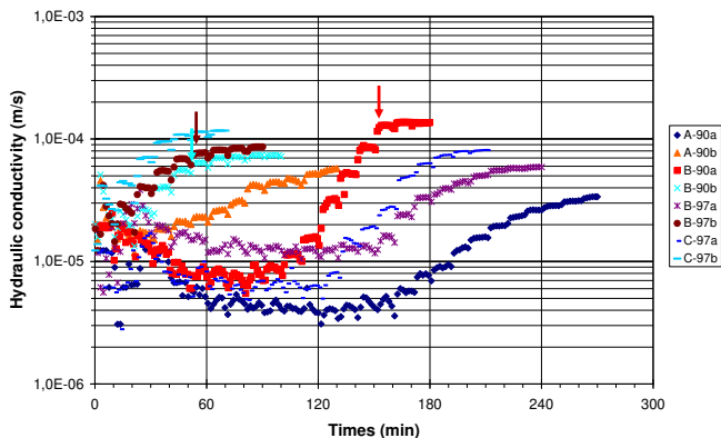
Figure 5. Variation of hydraulic conductivity
