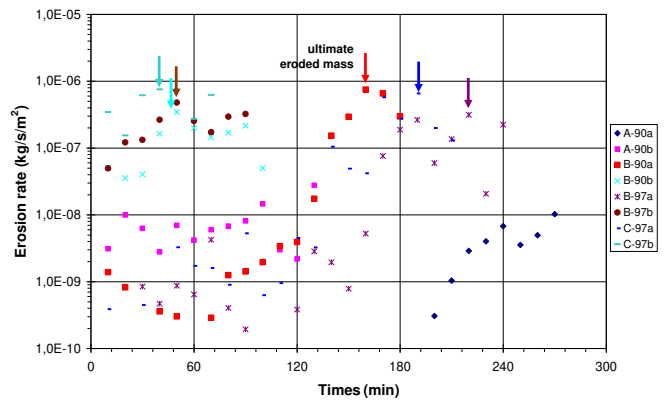
Figure 6. Variation of erosion rate during elapsed time
