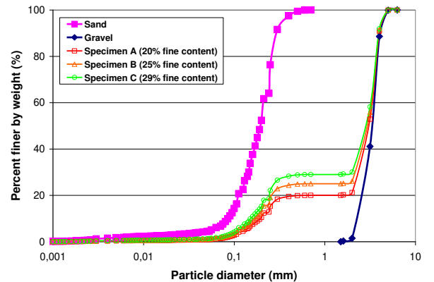
Figure 2. The particle size distribution of tested gradations
