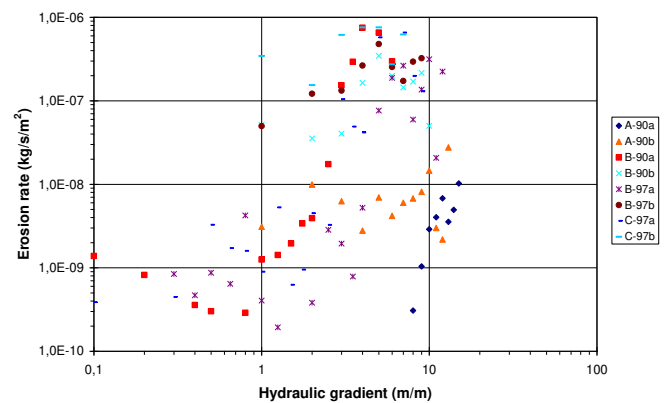
Figure 7. Variation of erosion rate to hydraulic gradient
