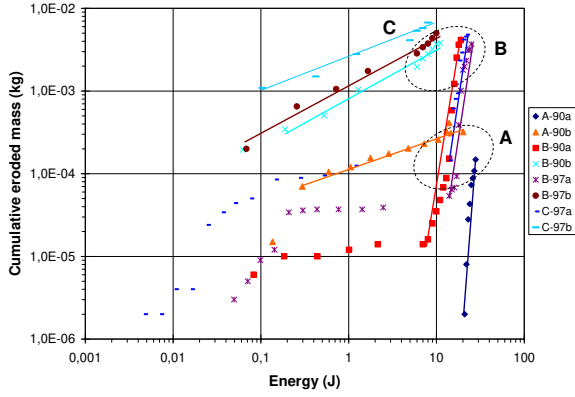
Figure 11. Cumulative eroded dry mass to cumulative expanded energy
