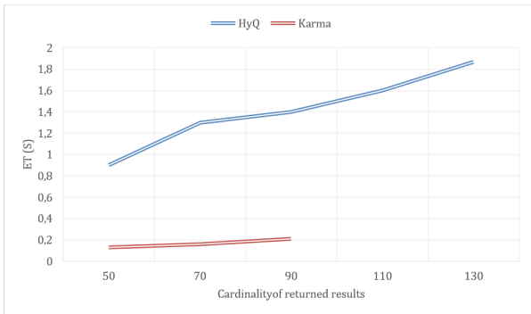
Figure 22: Performance variation in terms of execution time and cardinality of returned results.
