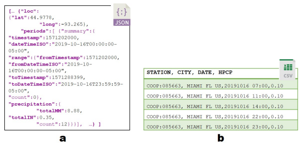
Figure 2: (a) Partial view of data about precipitation from the AeriWeather API. (b) Partial view of data about Hourly Precipitation (HPCP) from the NOAA. Data schema in bold.
