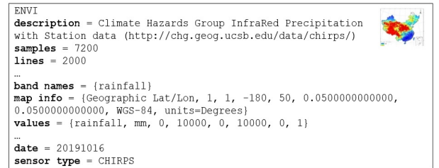
Figure 1: Partial view of the metadata from the raster image originating from the OSS.
