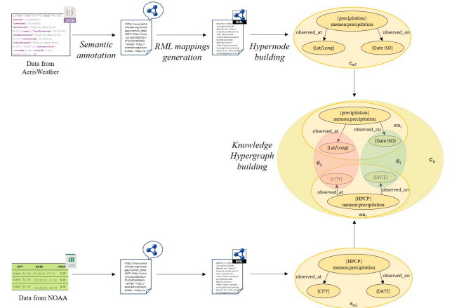
Figure 8: The process of the virtual integration from data to knowledge hypergraph building.
