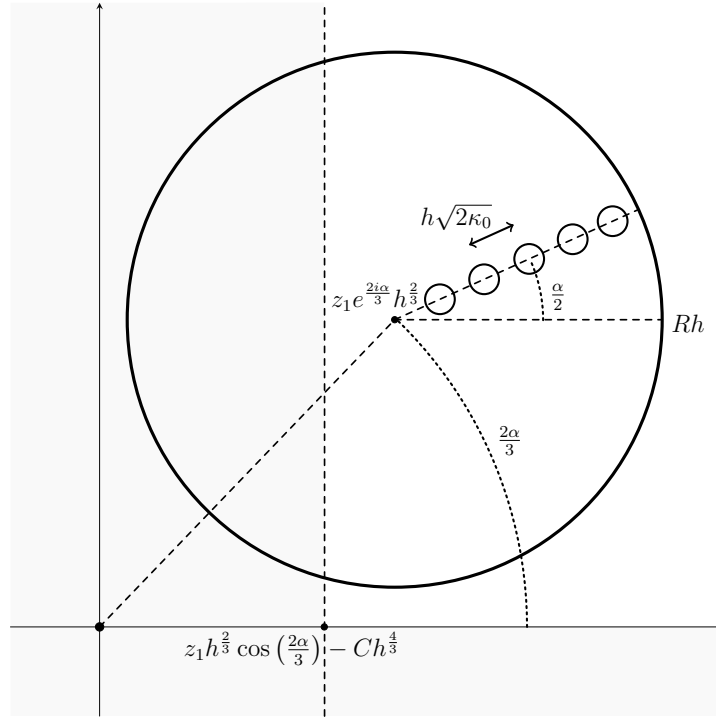
FIGURE 1. The spectrum in the disk of center z_1 e^{\frac{2i\alpha}{3}} h^{\frac{2}{3}} and radius Rh , when \alpha \in [0, \frac{3\pi}{5}) .
