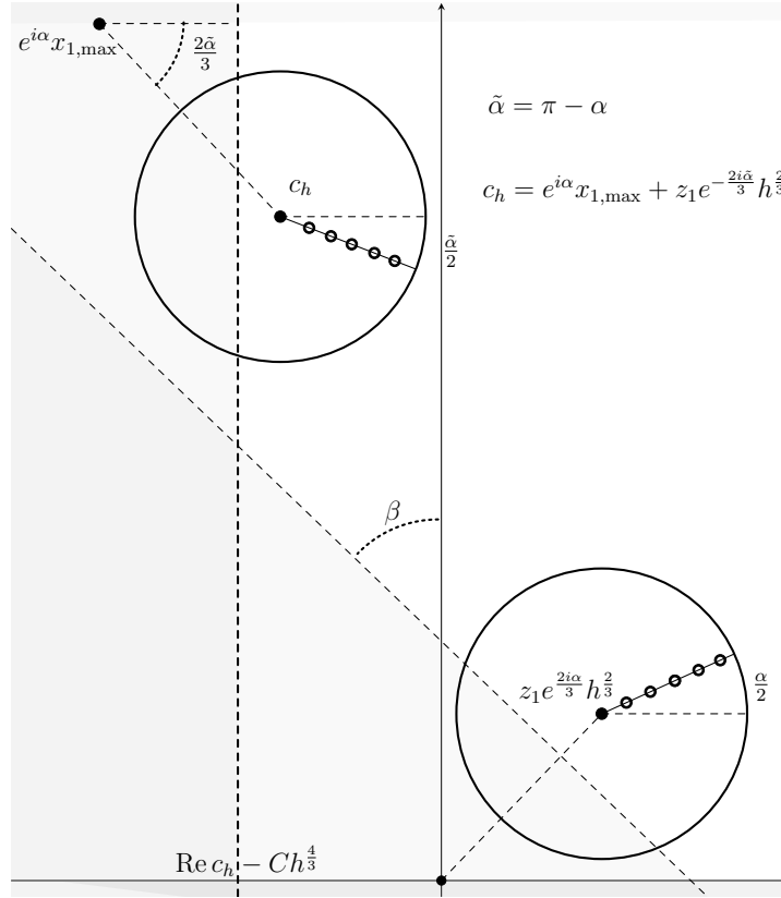
FIGURE 2. Case when \alpha \in (\frac{\pi}{2}, \frac{3\pi}{5}) .
