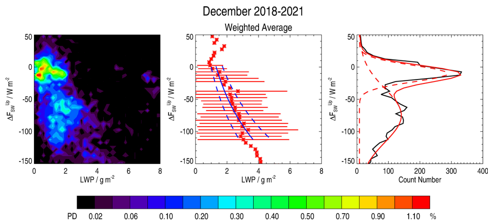
Figure 9. As in Fig. 5 but for \Delta F_{SW}^{Up} .
