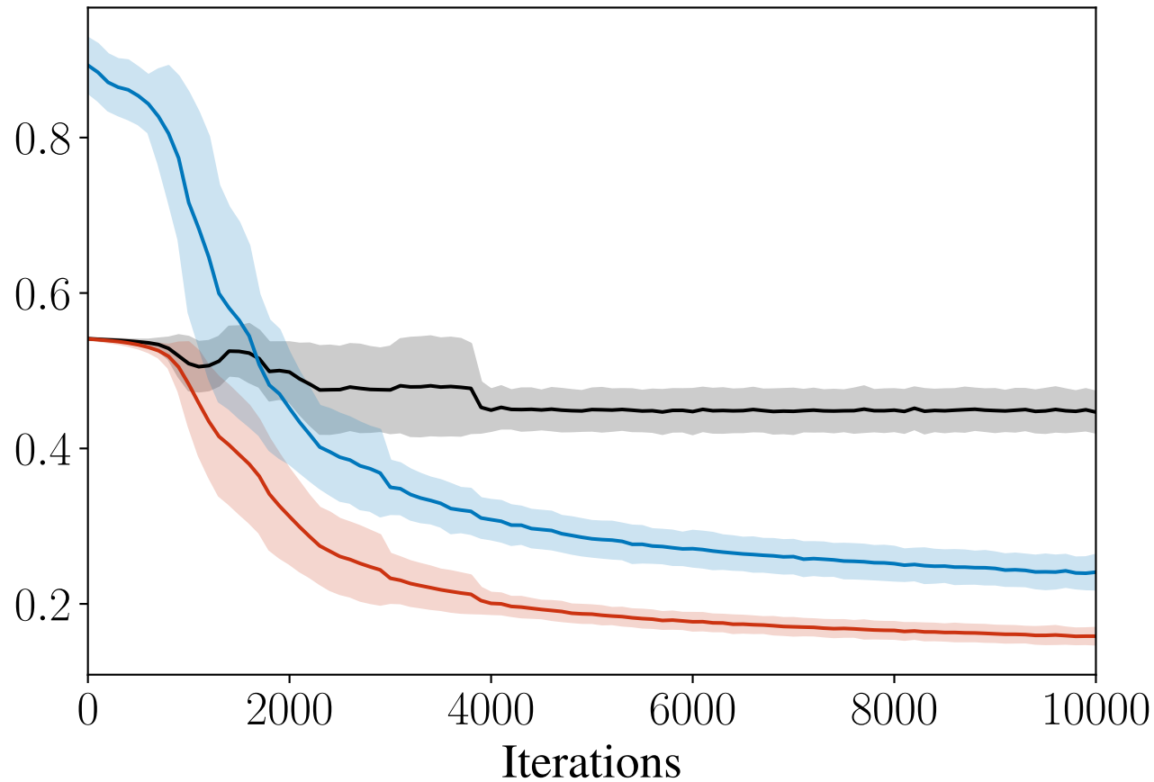
FashionMNIST
