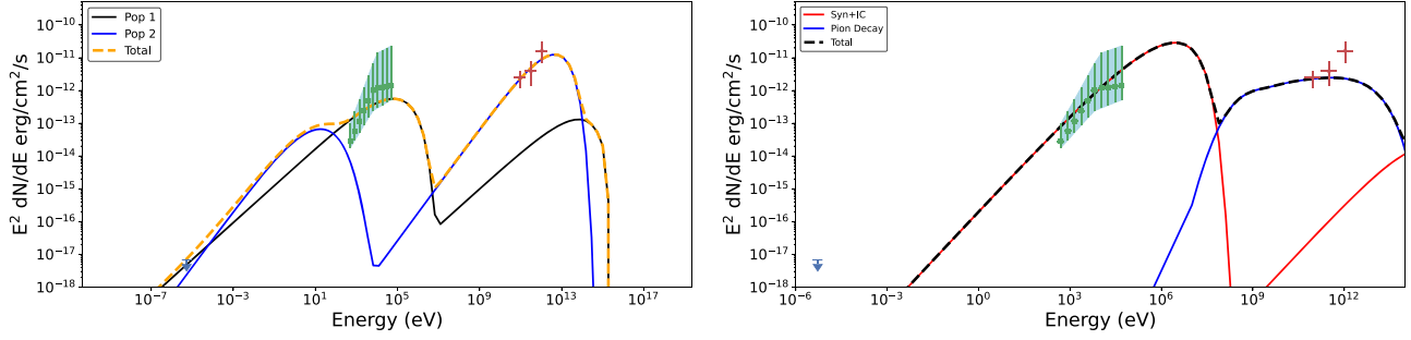
Figure 10. Broadband representations for the radio, X-ray, and 2FHL \gamma -ray data combination. (Left) Best-fit broadband model for the leptonic scenario. Radio data is taken from Heywood et al. (2022), X-ray data is from this work, and Fermi-LAT data from Ackermann et al. (2016), Ajello et al. (2017). (Right) Best-fit broadband model for the lepto-hadronic scenario.
