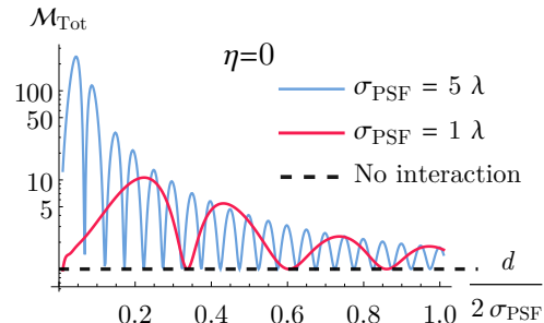
FIG. 10. Normalized total sensitivity \mathcal{M}_{Tot} (52) of two dipoles' separation estimation vs. separation d . The red line corresponds to \sigma_{PSF} = \lambda , the blue line to \sigma_{PSF} = 5\lambda , and the dashed line to non-interacting dipoles. No dephasing ( \eta = 0 ).
