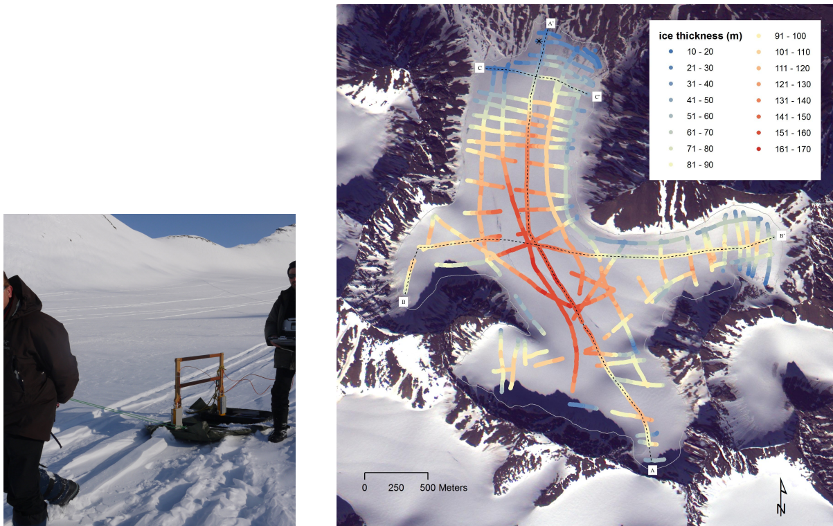
Figure 1 Right: Ice thickness map (from Saintenoy et al. (2013)) derived from GPR data set acquired with an old generation GPR system (left).
