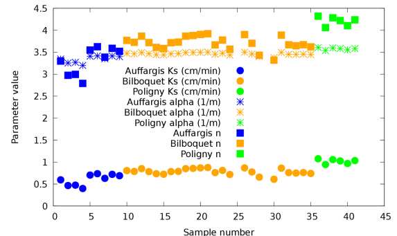
Figure 3: Hydrodynamical parameters estimated with Rosetta from granulometric measurements of Fig.2
