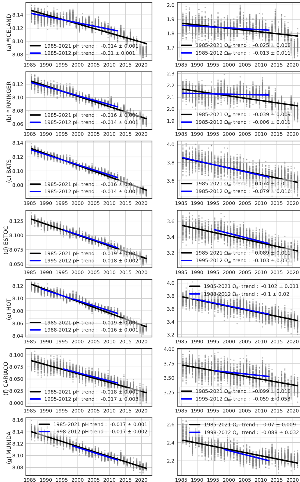
Figure A14. Linear trend estimates (per decade) learnt on 100-member ensembles (grey points) of yearly mean time series of pH and \Omega_{ar} at different stations (Bates et al., 2014). \mu \pm \sigma present linear slope and residual standard deviation. Black or blue lines stand for linear fits over the full or sub-period in 1985–2021 (see Table 5 for comparison).
