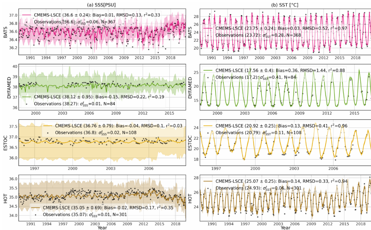
Figure A10. Monthly time series of SSS and SST at BATS, DYFAMED, ESTOC, and HOT stations (Table 2 and Fig. A1b): CMEMS data (curve), 1\sigma uncertainty (envelope), and monthly average of observations (point). Means of CMEMS data and 1\sigma uncertainty ( \mu \pm \sigma ) calculated over the observation time span are shown in brackets if accessible. Statistics include the number of months with observations ( N ), bias, RMSD, and r^2 ; \sigma_{SSS}^t ( \sigma_{SST}^t ) stands for temporal standard deviation from monthly averages of SSS and SST observations. Temporal variations in SSS observations are poorly described in the CMEMS SSS time series (Table 1) used in CMEMS-LSCe reconstructions.
