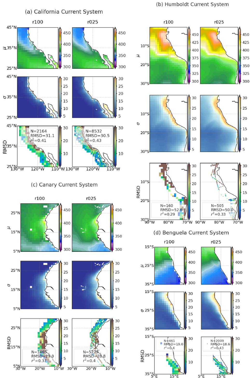
Figure 2. Comparison of CMEMS-LSCE-FFNN mapping p\text{CO}_2 at 1^\circ ( r100 ) and 0.25^\circ ( r025 ) resolutions over four permanent upwelling regions associated with the eastern boundary currents (California, Humboldt, Canary, and Benguela; see Fig. A1 (A, B, G, and H) for geographical locations). For each region, spatial distributions of p\text{CO}_2 ( \mu ) and uncertainty ( \sigma ) estimates and the coastal–ocean RMSD of p\text{CO}_2 averaged over 1985–2021 (Eqs. 5 and 10) are shown. Metrics presented in the legend for each of the third rows include the number of coastal–ocean SOCATv2022 data ( N ), regional RMSD (Eq. 10), and r^2 (Eq. 11).
