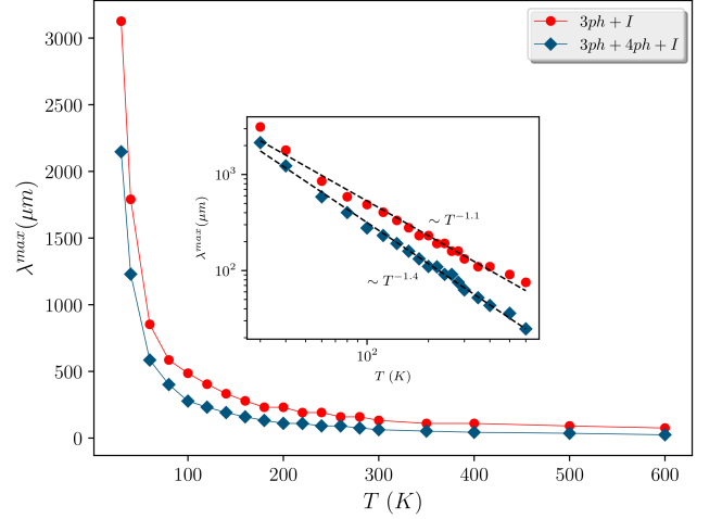
FIG. 12. The variation of maximum mean free path ( \lambda^{max} ) as a function of temperature for \text{Ge}_2\text{Sb}_2\text{Te}_5 both including and excluding 4ph scattering. Inset shows the scaling relation of \lambda^{max} with T with (3ph+4ph+I) or without (3ph+I) 4ph scattering.
