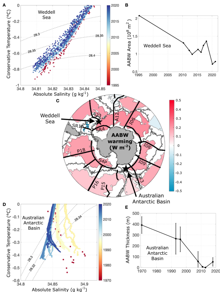
FIGURE 6 Decadal variability of Antarctic Bottom Water (AABW) properties from repeat hydrographic data. (A) Conservative temperature (°C) versus absolute salinity (g/kg) diagram in the Weddell Sea from measurements collected along the A23 line south of 60°S (see black star in panel C for location). (B) AABW area (m 2 ) along the A23 line south of 60°S (Abrahamsen et al., 2019; Zhou et al., 2023; neutral density >28.4 kg/m 3 ). (C) AABW warming (W/m 2 ) between the 1990s and the 2010s (see Purkey and Johnson, 2010, for methodology; >4,000 m depth). (D) Conservative temperature versus absolute salinity plot in the Australian Antarctic Basin obtained by observations along the P11S line at 150°E (see black star in panel C for location). (E) AABW (neutral density >28.34 kg/m 3 ; Silvano et al., 2020) thickness (m) along 150°E. AABW density varies in different sectors and therefore AABW definitions change accordingly. GO-SHIP sections are depicted in black in (C).
