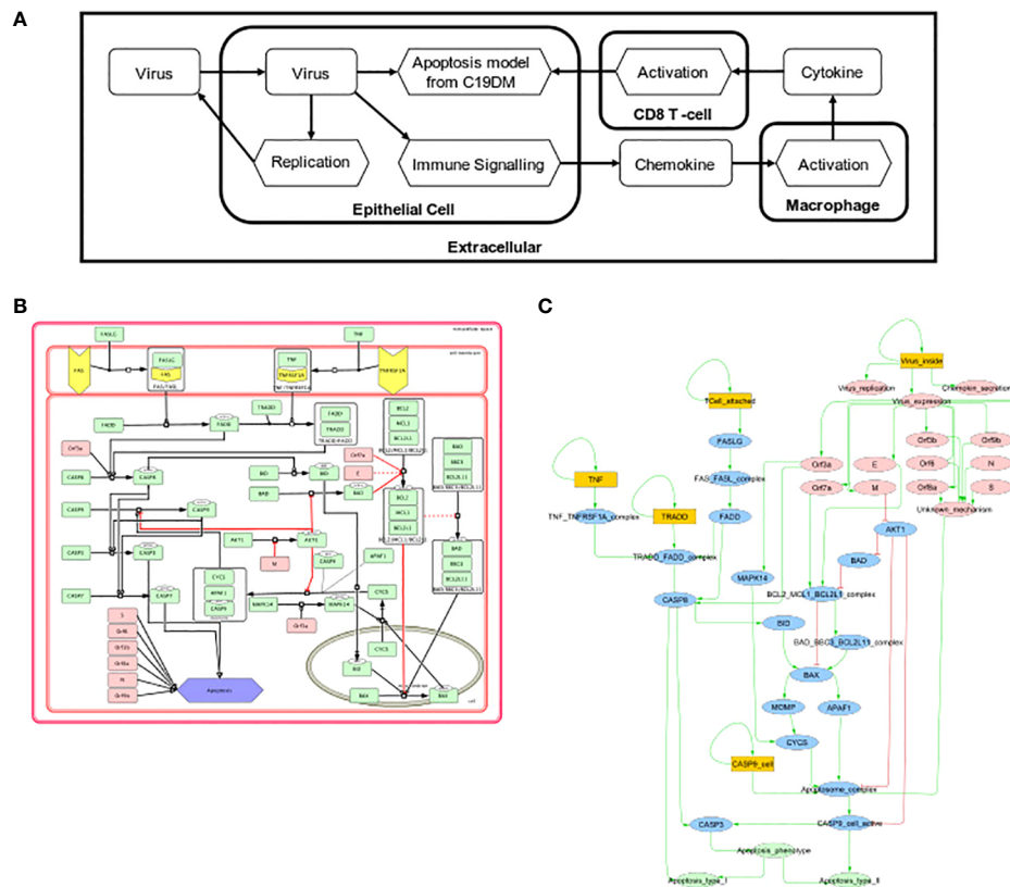
FIGURE 7 Multiscale simulation workflow. (A) Overview of the top-level interaction model that integrates virus infection, host respiratory epithelial cell demise, and the response of different immune cells. (B) The apoptosis model from C19DMMap ( https://fairdomhub.org/models/712 ). (C) The modified version of the apoptosis model was included in each respiratory epithelial cell type.
