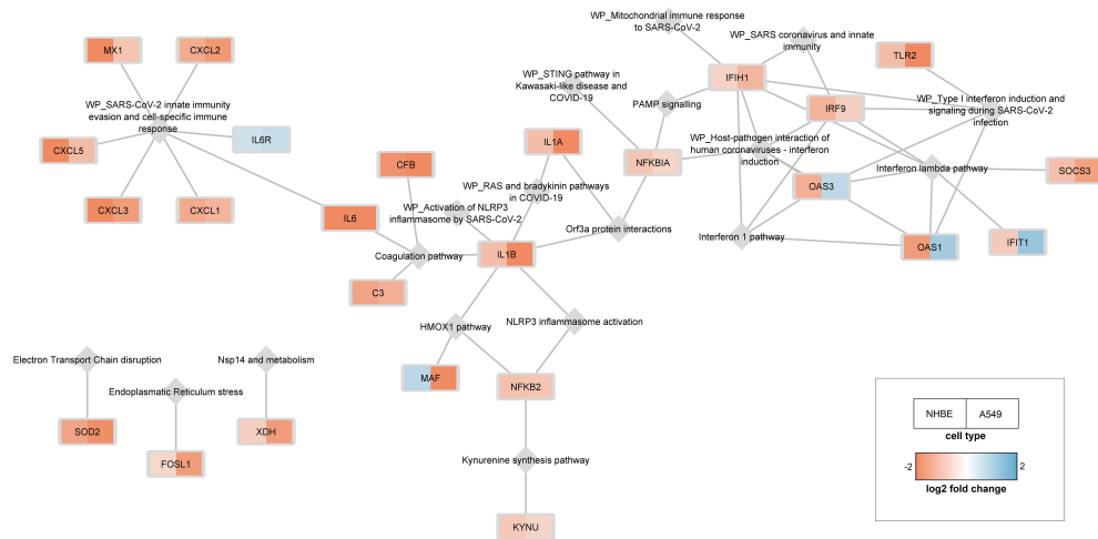
FIGURE 3 25 genes differentially expressed in both cell lines are linked to 19 pathways. C19DMap pathways are represented as grey diamonds, and shared DEGs are coloured as rectangles following expression fold change.
