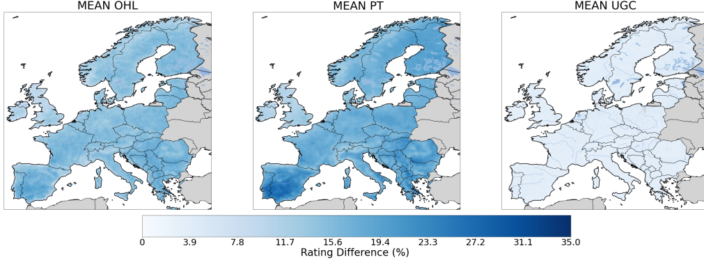
Figure 2: Geographical distribution of the mean Historical \Delta\%(qDTR_H, STR_H) difference at the country level. This is performed for the three main power components (OHL, PT and UGC).
