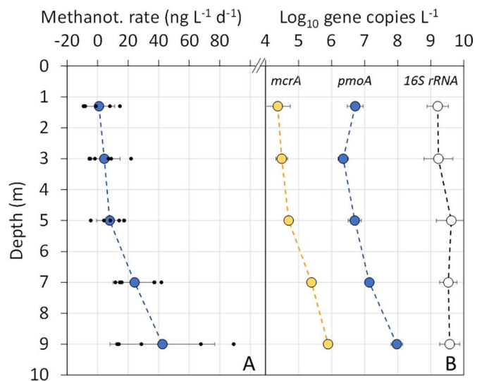
Fig. 4. (A) Methanotrophic rates and (B) gene copy number observed in the watercolumn of lake Kitiash (L2) during the ice-season. Each point represents the mean of four replicates and standard deviations are shown. mcrA and pmoA genes are marker genes of methanogens and methanotrophs, respectively. Note that the 16S rRNA gene copy number corresponds to the sum of both bacterial and archaeal 16S rRNA gene copies, representing all prokaryotes (Table S2).
