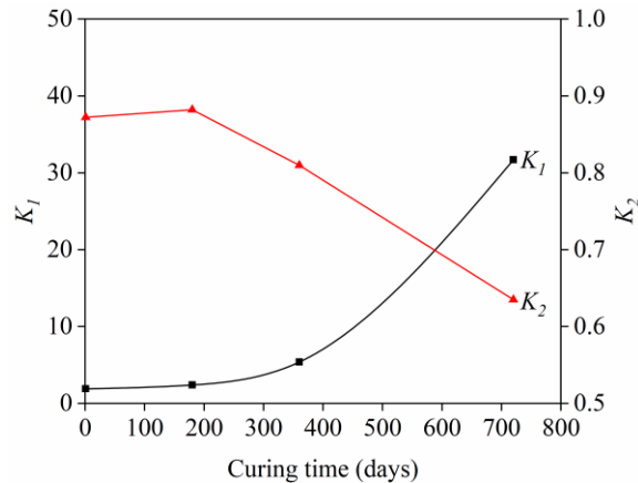
Figure 9. Evolution of k - \theta model parameters K_1 and K_2 of NRCA with curing time
