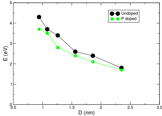
Fig. 3 Position in energy, with respect to the HOMO (set equal to zero), of the P related impurity state (green squares) and of the LUMO state for the undoped Si-NCs (black dots), as function of the NC diameter.
