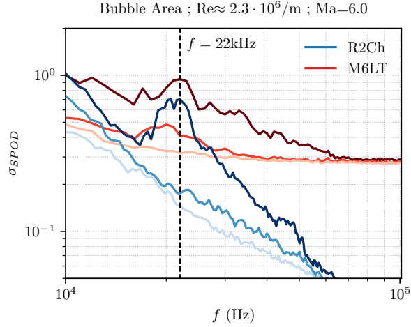
Fig. 19 Normalized SPOD energy around the bubble area for the three first rank at Re_\infty = 2.2 \times 10^6/m .
