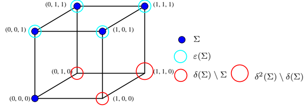
Figure 7. Illustration of the morphological ordering (here n = 2, m = 1 ), using B^{ab} as structuring element.
