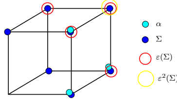
Figure 12. An example of last consistent erosion.
