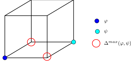
Figure 11. Example of merging \Delta^{max}(\varphi, \psi) , obtained for a dilation of size n = 1 .
