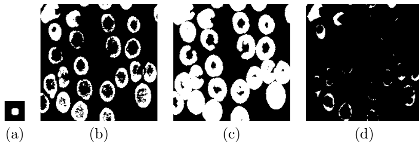
Figure 1. (a) Structuring element B (ball of the Euclidean distance). (b) Subset X in the Euclidean plane (in white). (c) Its dilation \delta_B(X) . (d) Its erosion \varepsilon_B(X) .
