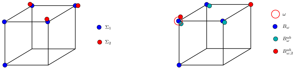
Figure 15. Illustration of \Sigma_1 and \Sigma_2 (left) and of three different structuring elements centered at \omega (right).
