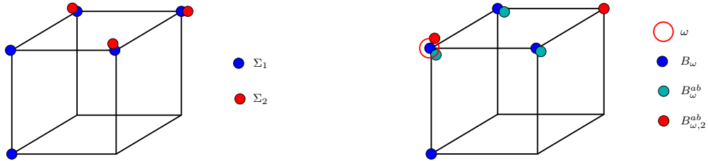
Figure 15. Illustration of \Sigma_1 and \Sigma_2 (left) and of three different structuring elements centered at \omega (right).
