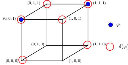
Figure 2. Example of a dilation of size 1: \varphi = (a \wedge b \wedge c) \vee (\neg a \wedge \neg b \wedge c) and \delta(\varphi) = (\neg a \vee b \vee c) \wedge (a \vee \neg b \vee c) . Note that in all figures, the models of the formulas are represented. Note that this figure and the next ones may be best seen in colors on the online version of the paper.
