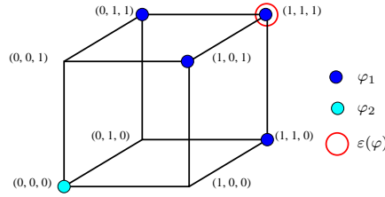
Figure 8. Decomposition of \varphi into two connected components \varphi_1 and \varphi_2 , and its erosion (only a , b and c are considered in this representation).
