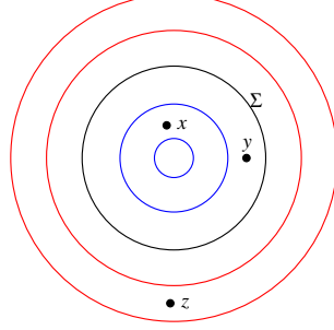
Figure 5. Illustration of a natural partial ordering derived from successive erosions (in blue) and dilations (in red) of \Sigma . We have x \preceq_f y \preceq_f z in this example.
