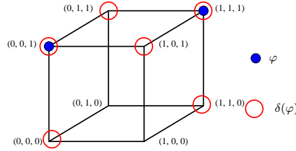
Figure 2. Example of a dilation of size 1: \varphi = (a \wedge b \wedge c) \vee (\neg a \wedge \neg b \wedge c) and \delta(\varphi) = (\neg a \vee b \vee c) \wedge (a \vee \neg b \vee c) . Note that in all figures, the models of the formulas are represented. Note that this figure and the next ones may be best seen in colors on the online version of the paper.
