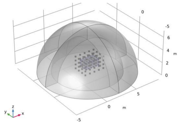
Figure 2. Geometry for the calculation of the direct pressure field where the 72 monopole point sources are regularly distributed in the blue box and the 62 minimization points are distributed all around.
