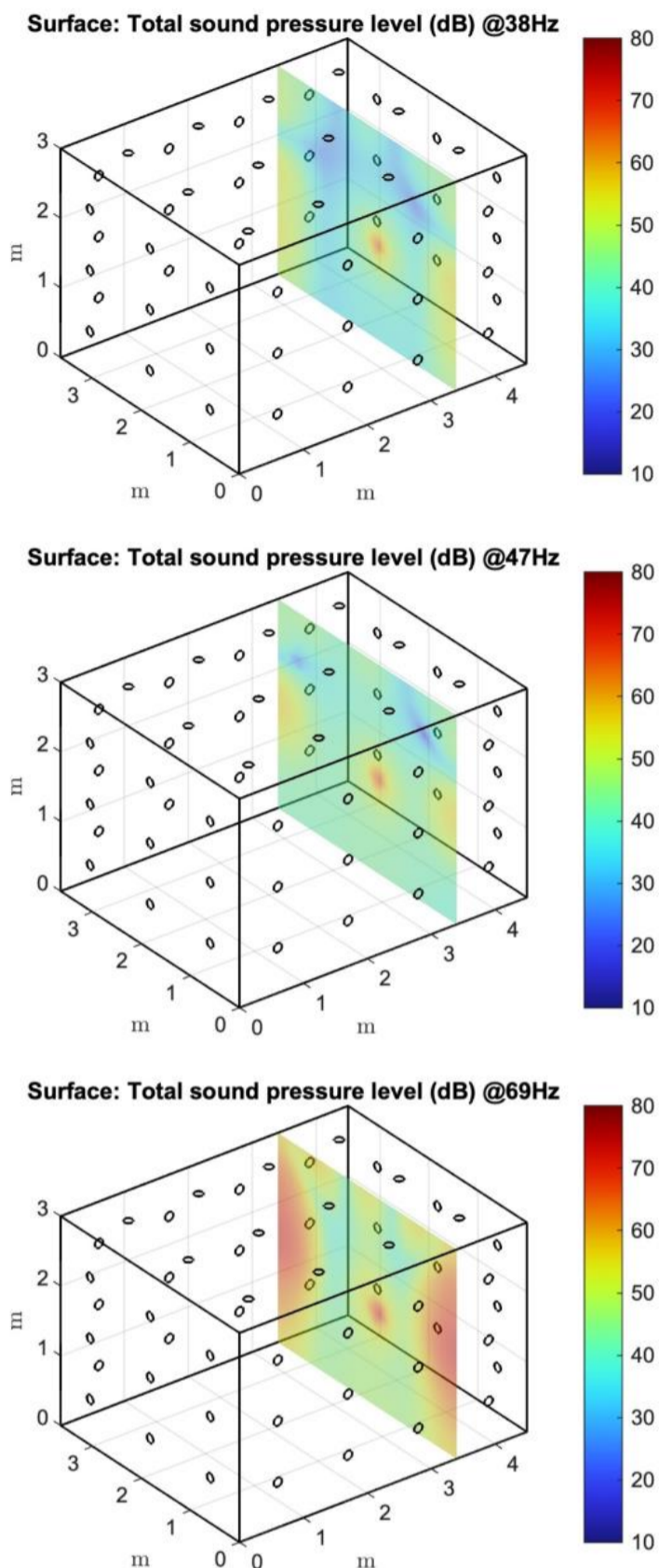
Figure 8. Slice plot showing how pressure is distributed inside the room with control the on at 38 Hz, 47 Hz and 69 Hz, in the yz-plane of the test source.
