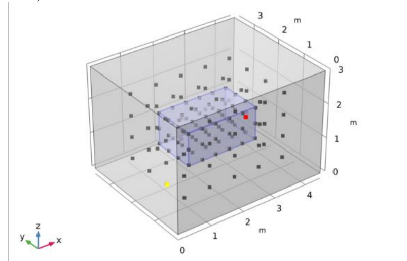
Figure 3. Geometry for the calculation of the total pressure field in the room where the 72 monopole point sources are distributed throughout the volume to be controlled (blue box) and the 62 minimization points are distributed all around.
