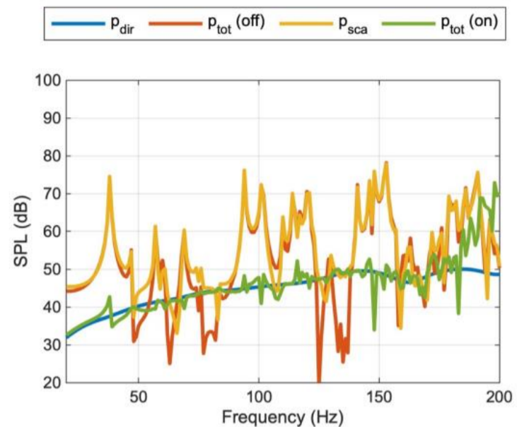
Figure 5. Room frequency response with control switched off/on
