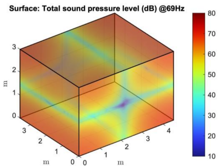
Figure 6. Total sound pressure level with the control off at 38 Hz, 47 Hz and 69 Hz.
