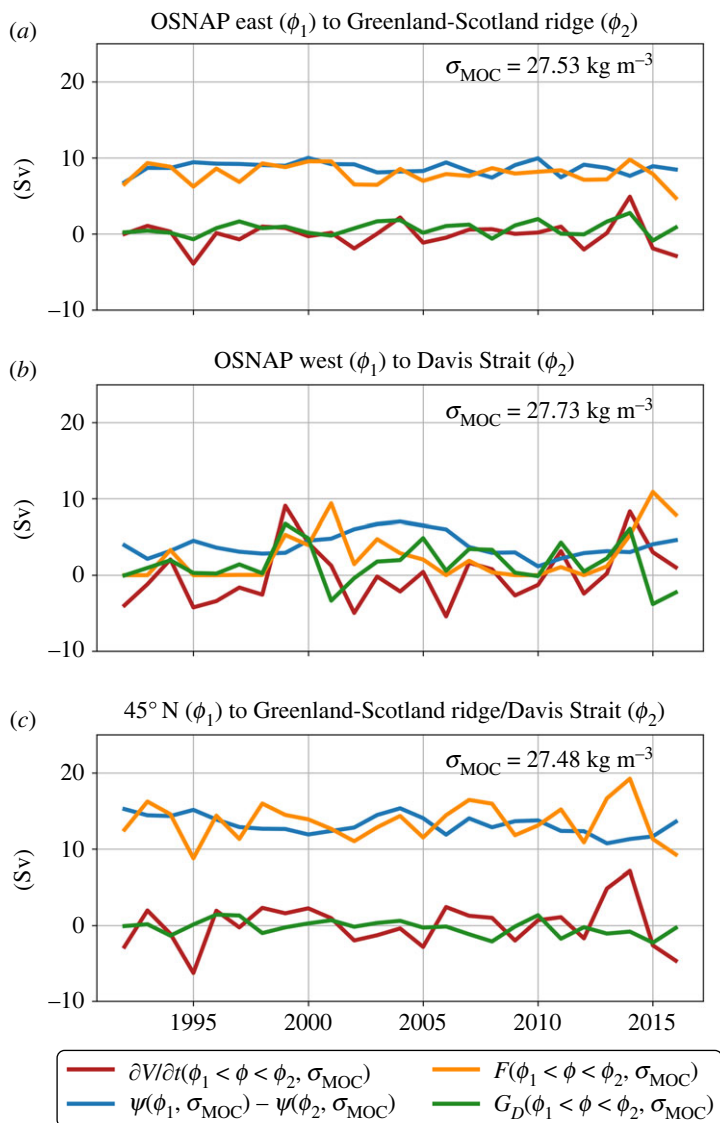
Figure 7. (a) Annual mean (June through May, to keep winter season contiguous) density/volume budget of the lower layer (below \sigma_{MOC} ) for (a) OSNAP East to the Greenland–Scotland Ridge, (b) OSNAP West to Davis Strait and (c) 45^\circ \text{ N} to the Greenland–Scotland Ridge/Davis Strait from Estimating the Circulation and Climate of the Ocean version 4 (ECCO v4) [10]. The plot shows the surface water mass transformation, F(\phi_1 < \phi < \phi_2, \sigma_{MOC}) (orange line); the overturning, \Psi(\phi_1, \sigma_{MOC}) - \Psi(\phi_2, \sigma_{MOC}) (blue line) and the volume change of the layer below isopycnal \sigma_{MOC} , \partial V/\partial t(\phi_1 < \phi < \phi_2, \sigma_{MOC}) (red line). The green line indicates the residual, which is interpreted as the water mass transformation due to mixing G_D(\phi_1 < \phi < \phi_2, \sigma_{MOC}) . \phi_1 and \phi_2 are the specific boundaries specified in (a–c). The values of \sigma_{MOC} for each region are listed in the top right of each figure.
