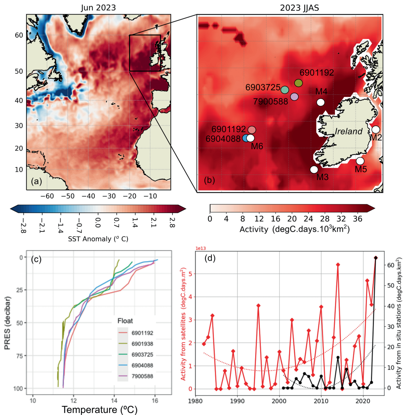
Figure 1. (a) Sea-surface temperature anomaly observed in June 2023 (degC) relative to 1982–2023. The black rectangle defines the study area (50–60°N, 20–5°W). (b) Activity of 2023 summer (June–July–August–September; JJAS) marine heatwave (MHW) (degC days 10 3 km 2 ) in study area. In situ observations from Irish meteorological buoys are shown in white open circles. Locations of Argo floats are shown with coloured open circles. (c) Depth profiles of the MHW based on Argo profiling float profiles from 11 to 15 June. Colours correspond to the locations in (b). (d) Times series of (red) satellite-derived summer (JJAS) and (black) buoy-derived June marine heatwaves mean activity. Dashed line represents the regression of a third-order polynomial. Daily sea-surface temperature (SST) data are from the NOAA Optimum Interpolation SST product (OISSTV2; Huang et al., 2020).
