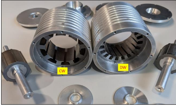
Fig. 7: DW and CW prototypes without winding and magnet
