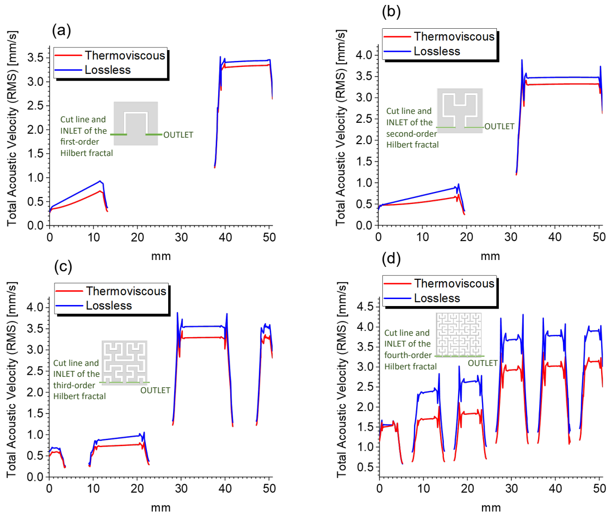
Figure S5. The four subfigures (a, b, c, d) show the total root mean square acoustic velocity in \text{mm/s} along a representative line passing through the middle of the inlet and outlet of metamaterials with w = 1\text{ mm} and n = 50.8\text{ mm} . Each subfigure presents two FEM simulations: one assuming lossless behavior within the small fractal pattern channels, and the other with a thermoviscous air model. Subfigure (a) illustrates the section line of the first-order Hilbert fractal, represented by a green segment. The absence of a velocity representation in parts of the graph corresponds to the solid portions of the fractal, where air is not present. This pattern is mirrored in subfigures (b), (c), and (d), which are related to the second, third, and fourth-order Hilbert fractals, respectively.
