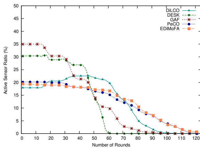
Fig. 3: Active sensors ratio for 200 deployed nodes.
