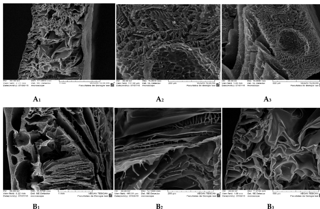
Figure 3. Scanning electron microscope (SEM) images for CS-PArg (A 1 –A 3 ) and CS-6h (B 1 –B 3 ) membranes at various magnifications of 1 mm, 200 \mu\text{m} , 500 \mu\text{m} .
