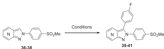
Scheme 2. Synthesis of fluorinated azindazoles. Reagents and conditions: 4-iodofluorobenzene (1.1 equiv), \text{Ag}_2\text{CO}_3 (1.0 equiv), \text{Pd}(\text{dppf})\text{Cl}_2 \cdot \text{CH}_2\text{Cl}_2 (0.05 equiv), \text{PPh}_3 (0.10 equiv), \text{H}_2\text{O} , 50^\circ\text{C} , 18 h, 39 : 4-aza 63%; 40 : 6-aza 75%; 41 : 7-aza 79%.
