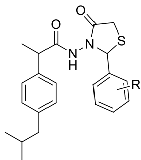
Fig. 1 The structure of ibuprofen derivatives with thiazolidine-4-one scaffold ( 4a-n )
