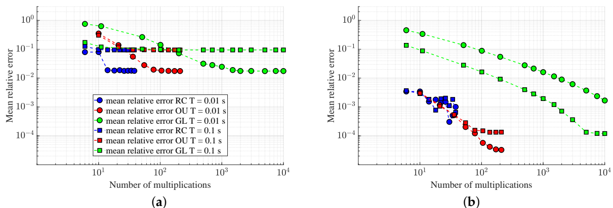
Figure 10. Average relative errors vs. numbers of multiplications for mRC, OU and GL. (a) Dynamic stage; (b) static stage.
