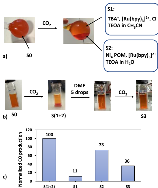
Fig. 3. Pictures of a) a 30 mL catalytic solution before and after bubbling \text{CO}_2 ; b) a 2 mL catalytic solution before and after bubbling \text{CO}_2 and after addition of DMF; c) normalized CO production of the various solutions. Catalytic conditions: 2 mL of \text{CO}_2 -saturated solution irradiated during 2 h (280 W Xe lamp, \lambda > 415 nm).
