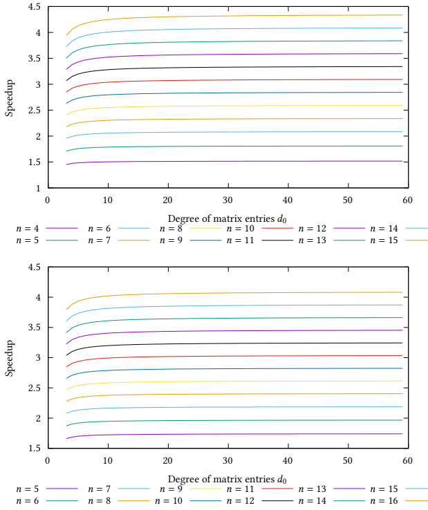
Figure 1: Speedup of Algorithm 1. Top: p = 3 ; bottom: p = 4
