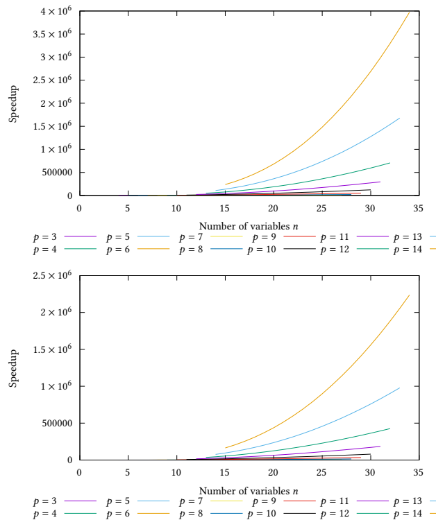
Figure 3: Speedup of Algorithm 1. Top: d_0 = 3 ; bottom: d_0 = 4 .
