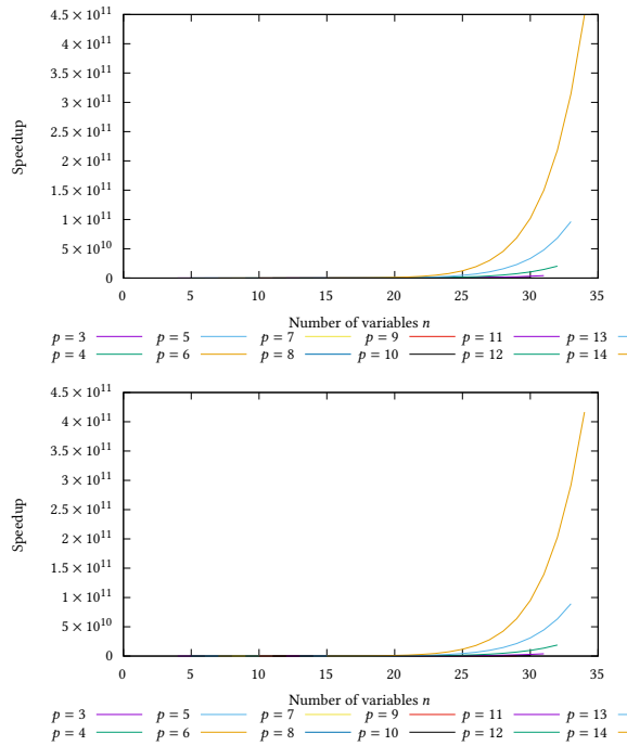
Figure 4: Speedup of an algorithm which computes full-rank Macaulay matrices. Top: d_0 = 3 ; bottom: d_0 = 4 .
