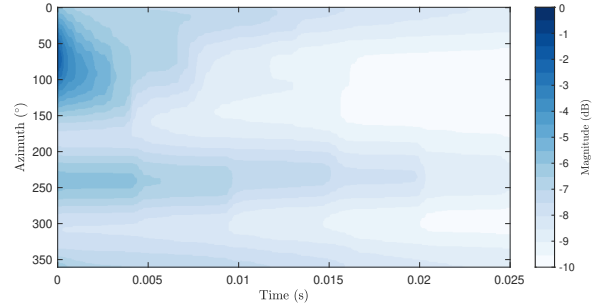
Figure 3. Directional EDC results on the horizontal plane, for the first 25 ms of an SRIR filtered between 1 kHz and 3 kHz, measured in front of seat 37, on the second row, using the first sound source.
