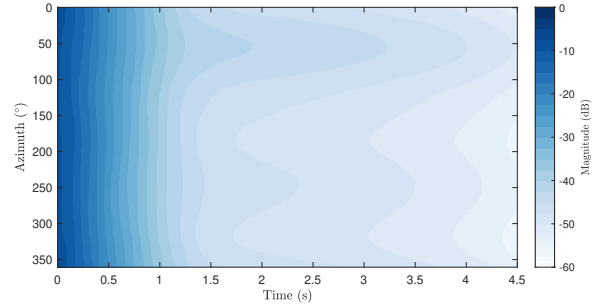
Figure 5. Directional EDC results on the horizontal plane, for the first 4.5 seconds of an SRIR filtered between 1 kHz and 3 kHz, measured in front of seat 37, on the second row, using the first sound source.
