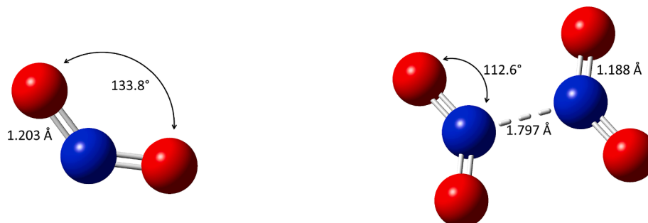
Fig. 4. Optimal geometry of \text{NO}_2 and \text{N}_2\text{O}_4 . Atomic coordinates are reported in Table S2 and S3 the Supporting Information.
