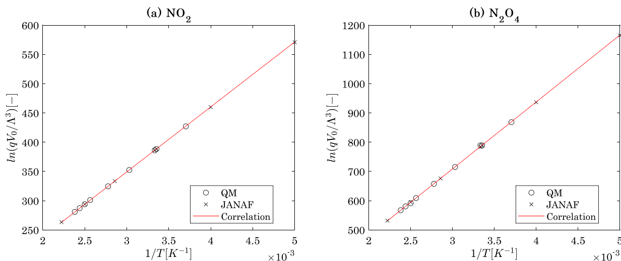
Fig. 3. Natural logarithm of the partition functions, q , divided by the thermal wavelength, for \text{NO}_2 (fig. (a)) and \text{N}_2\text{O}_4 (b). Data obtained from the JANAF tables. Correlations are eqs. (24) and (25).
