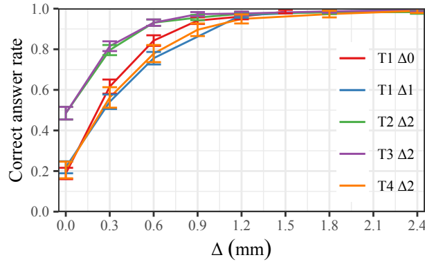
Fig. 7. Correct answer rates for the different values of the augmented size of the tallest segment.
