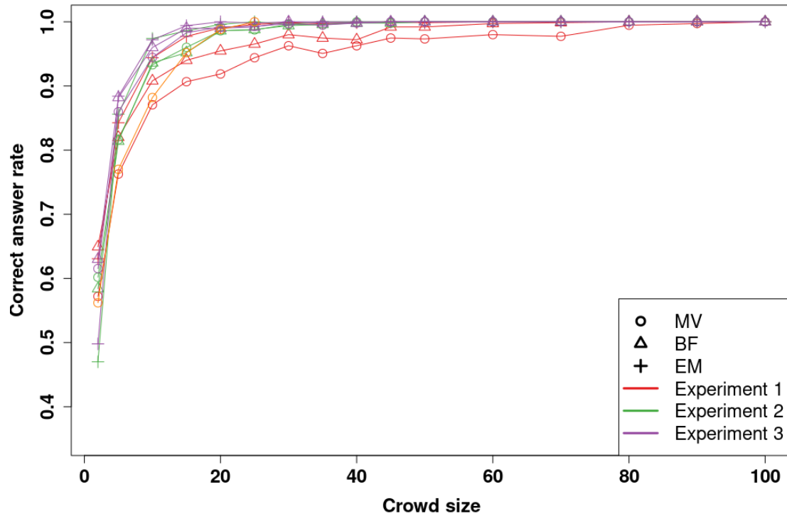
Fig. 8. Correct answer rate for \delta = 0.3 questions increasing the number of contributors selected to constitute the crowd.
