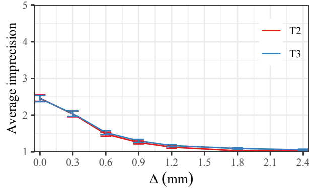
Fig. 6. Average imprecision of the answer for the different values of the augmented size of the tallest segment.
