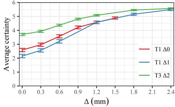
Fig. 5. Average certainty on the answer for the different values of the augmented size of the tallest segment. Error bars are 95% confidence intervals.
