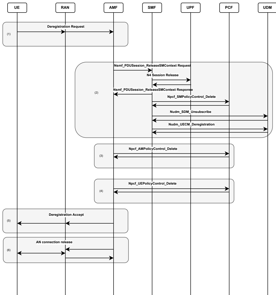
Figure 4: UE Deregistration Procedure
