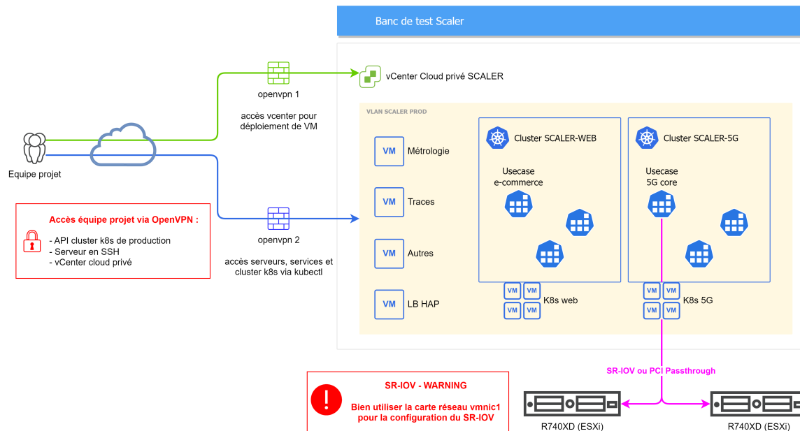
Figure 7: Eolas SCALER Testbed Architecture
