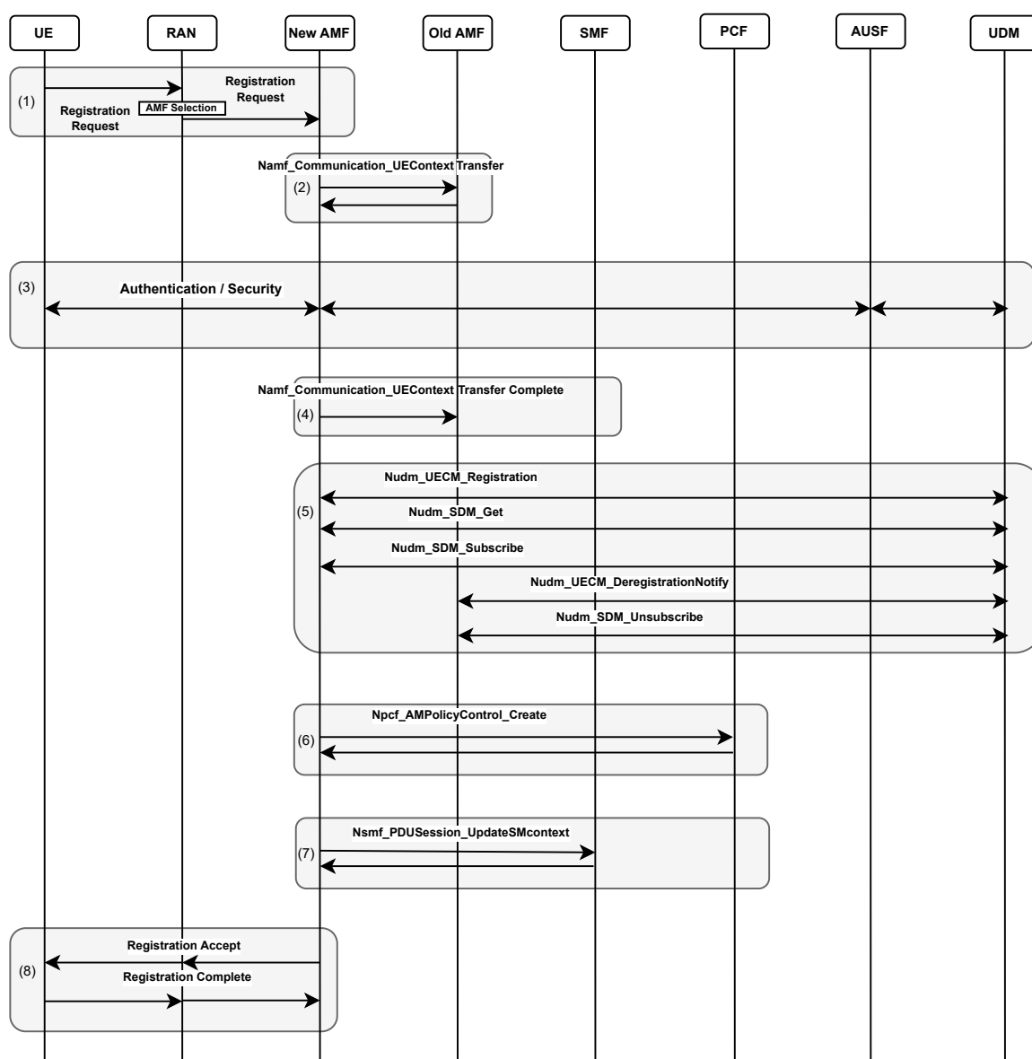
Figure 2: UE Registration Procedure
