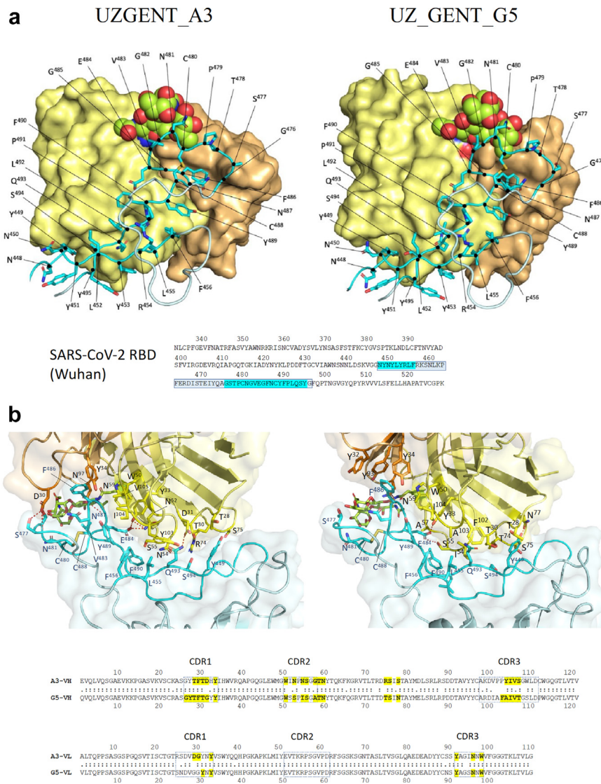
Fig. 9: Structures of the SARS-CoV-2 Spike with the UZGENT_A3 and UZGENT_G5 Fabs. (a) Closeup view of the UZGENT_A3 (left) or UZGENT_G5 (right) VH (yellow) and VL (orange) domains shown in solvent accessible surface representation, in complex with the SARS-CoV-2 RBD binding epitope (cyan; residues 449–497) shown in stick representation. The N59 glycosylation is shown in sphere representation. (b) Detailed view of the Spike–Fab epitope–paratope interface, shown in stick representation (coloured as in panel a). Bottom, amino acid sequence of the UZGENT_A3 and UZGENT_G5 VH and VL domains, with residues involved in binding interactions with the RBD highlighted in yellow.
