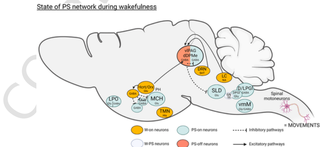
Fig. 2. State of PS network during wakefulness.
