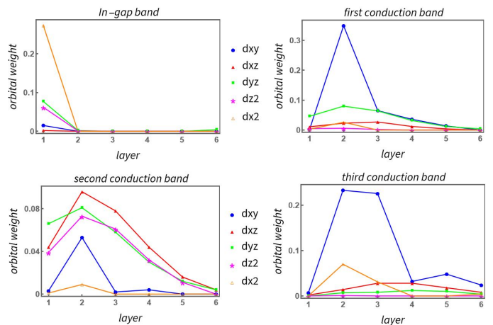
FIG. 6: d-orbital weights at \Gamma in a slab with a di-vacancy. For a given band (we show the in-gap and three lowest in energy) we extract the weights of the five d-orbitals components of the eigenfunction, projected onto each of the six \text{TiO}_2 layers.
