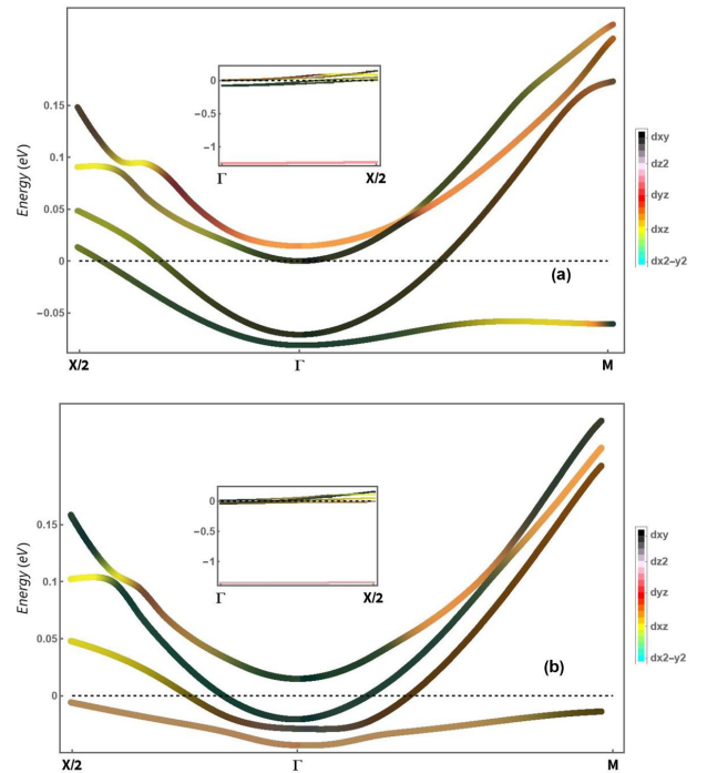
FIG. 3: Energy dispersion of conduction band states along a X - \Gamma - M path when di-vacancies are present close to the CaO termination (a) a slab with a horizontal di-vacancy at the CaO surface and (b) a slab with an apical di-vacancy in one of the (L6 layer) \text{TiO}_2 octahedra. Energies are measured relatively to E_F which is conventionally set to zero (dashed line). At every k-point the dominant orbital character of a given band eigenstate is indicated by a color which is assigned to each of the five d orbitals (see color chart). For instance, black color corresponds to d_{xy} , orange color for comparable weights of d_{xz} and d_{yz} . Insets in (a) and (b) display the e_g character in-gap state located \sim 1.3 eV below E_F .
